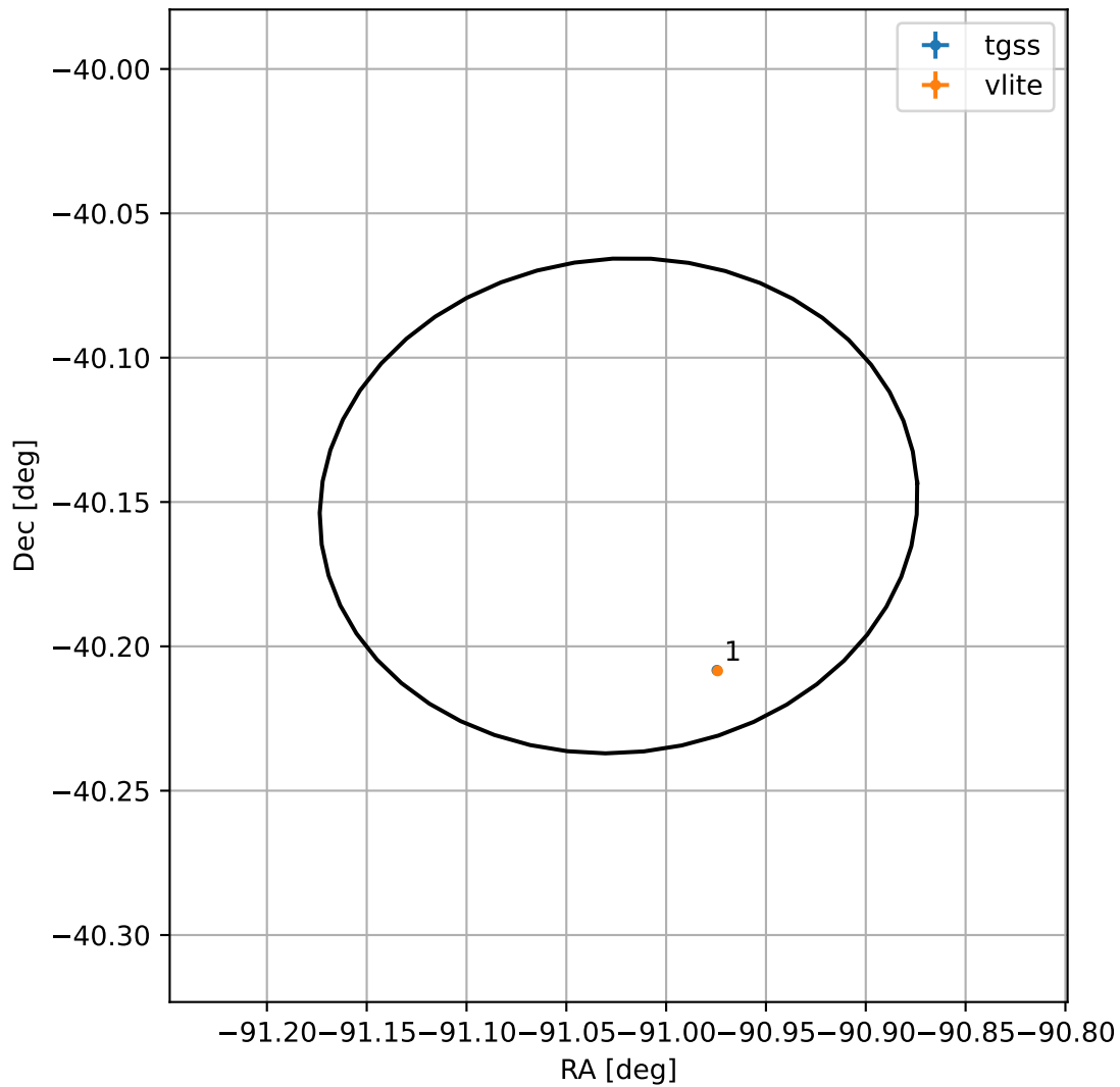
4FGL J1755.9-4009
