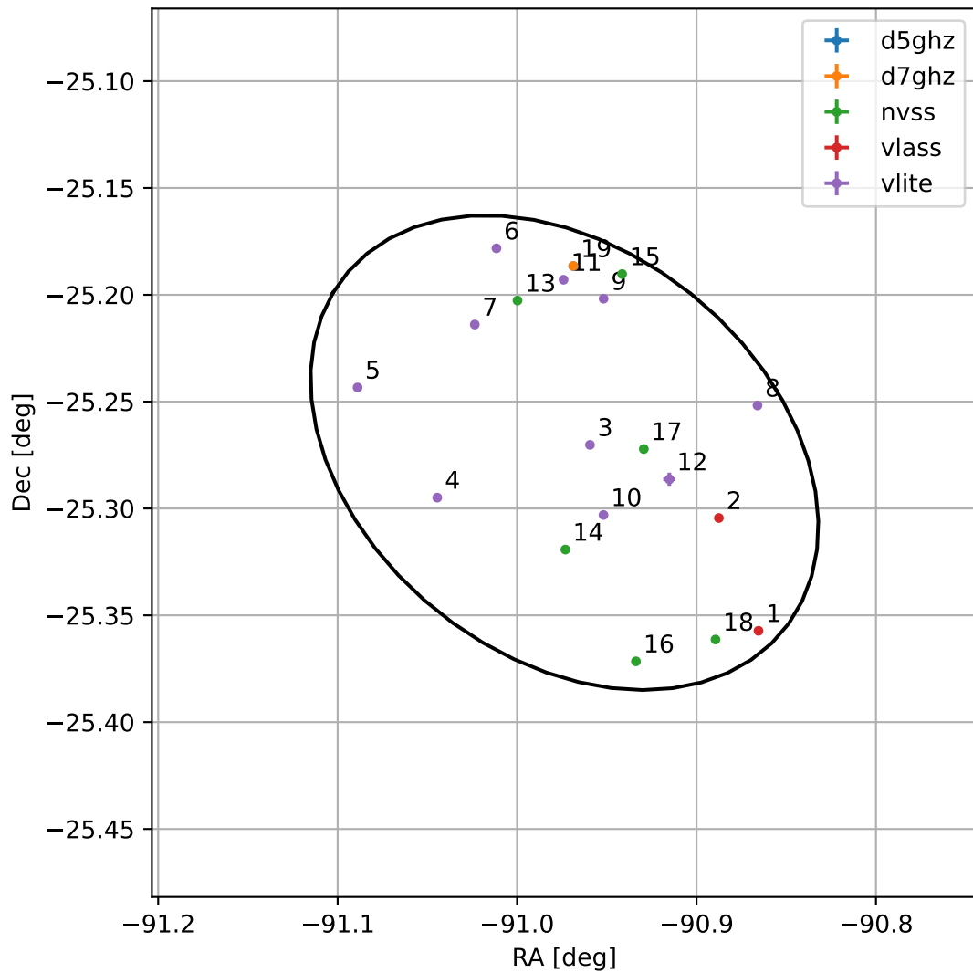
4FGL J1756.1-2516
