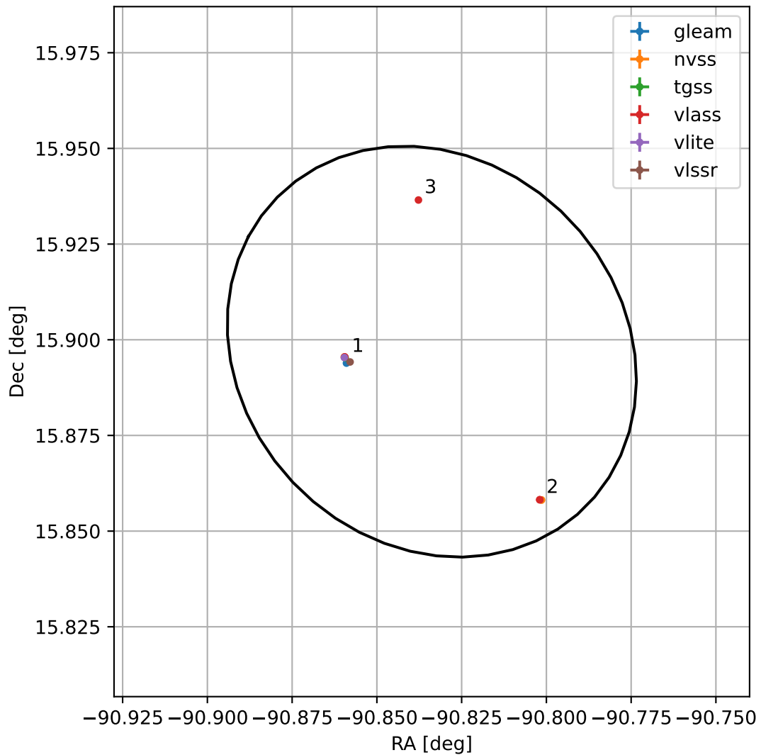
4FGL J1756.6+1553
