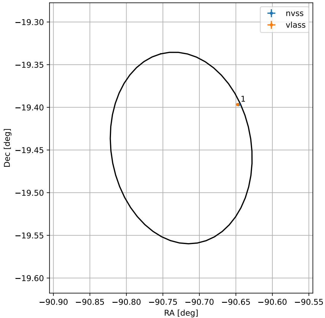
4FGL J1757.1-1926
