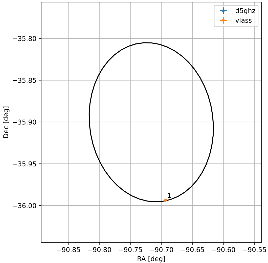
4FGL J1757.1-3554
