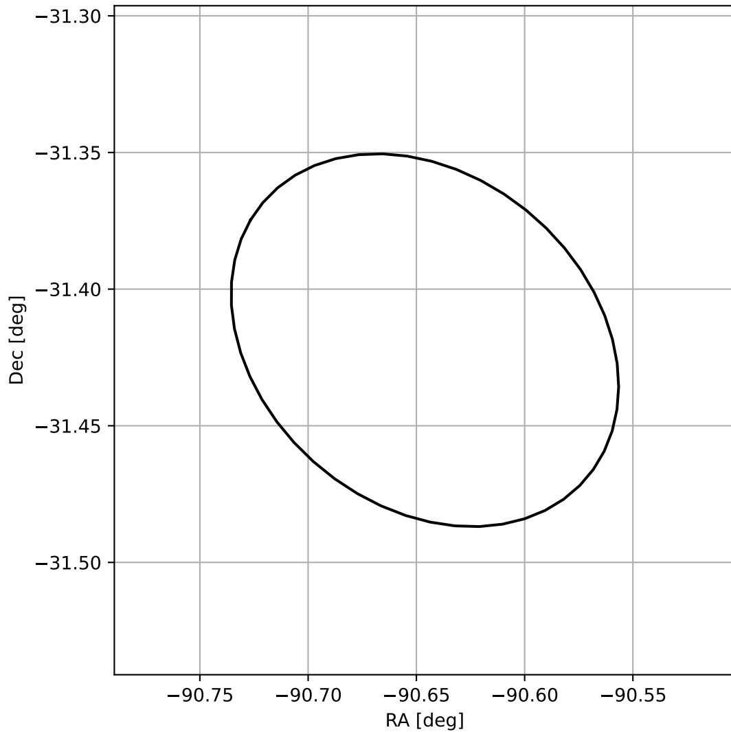
4FGL J1757.4-3125
