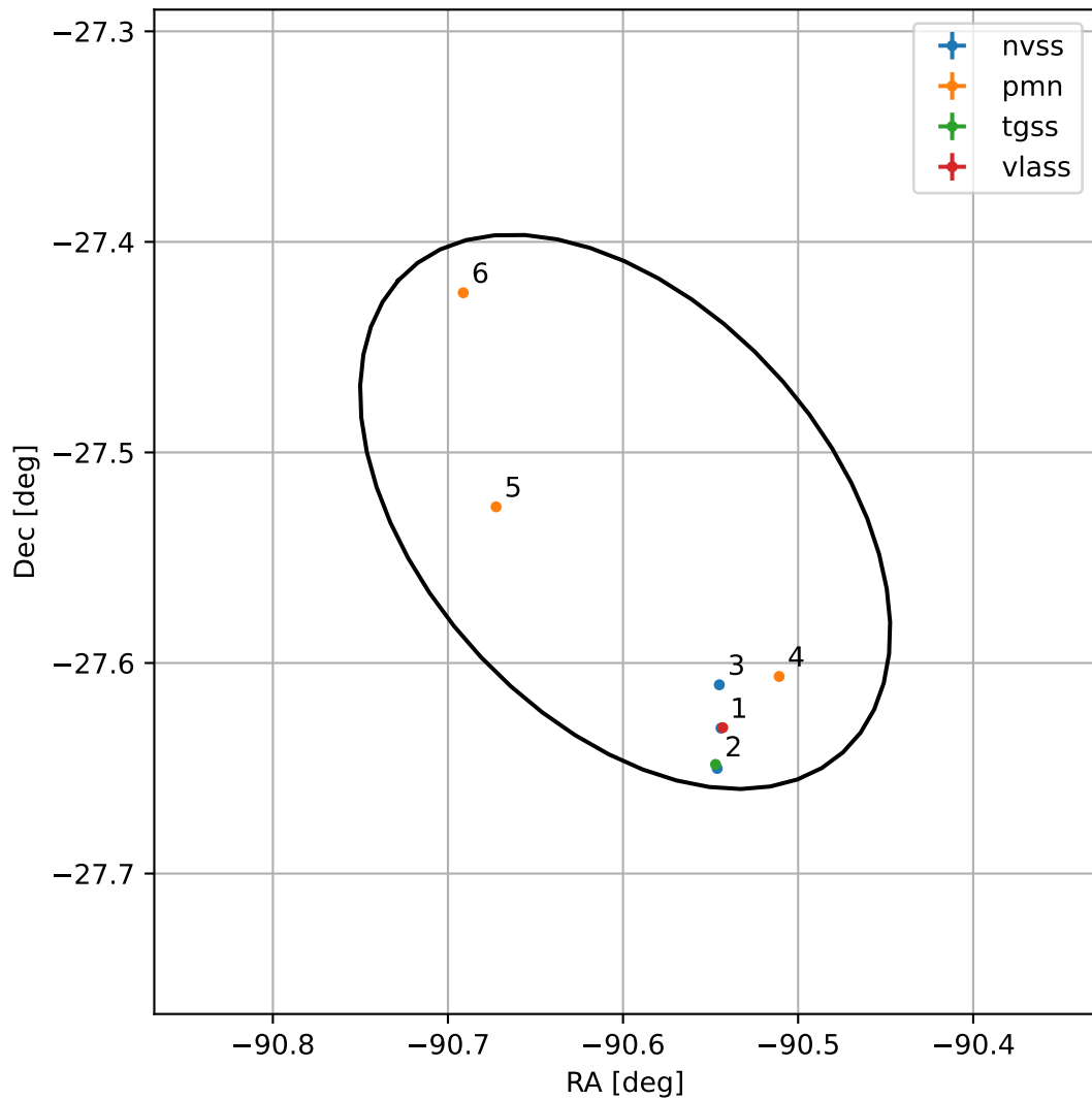
4FGL J1757.6-2731
