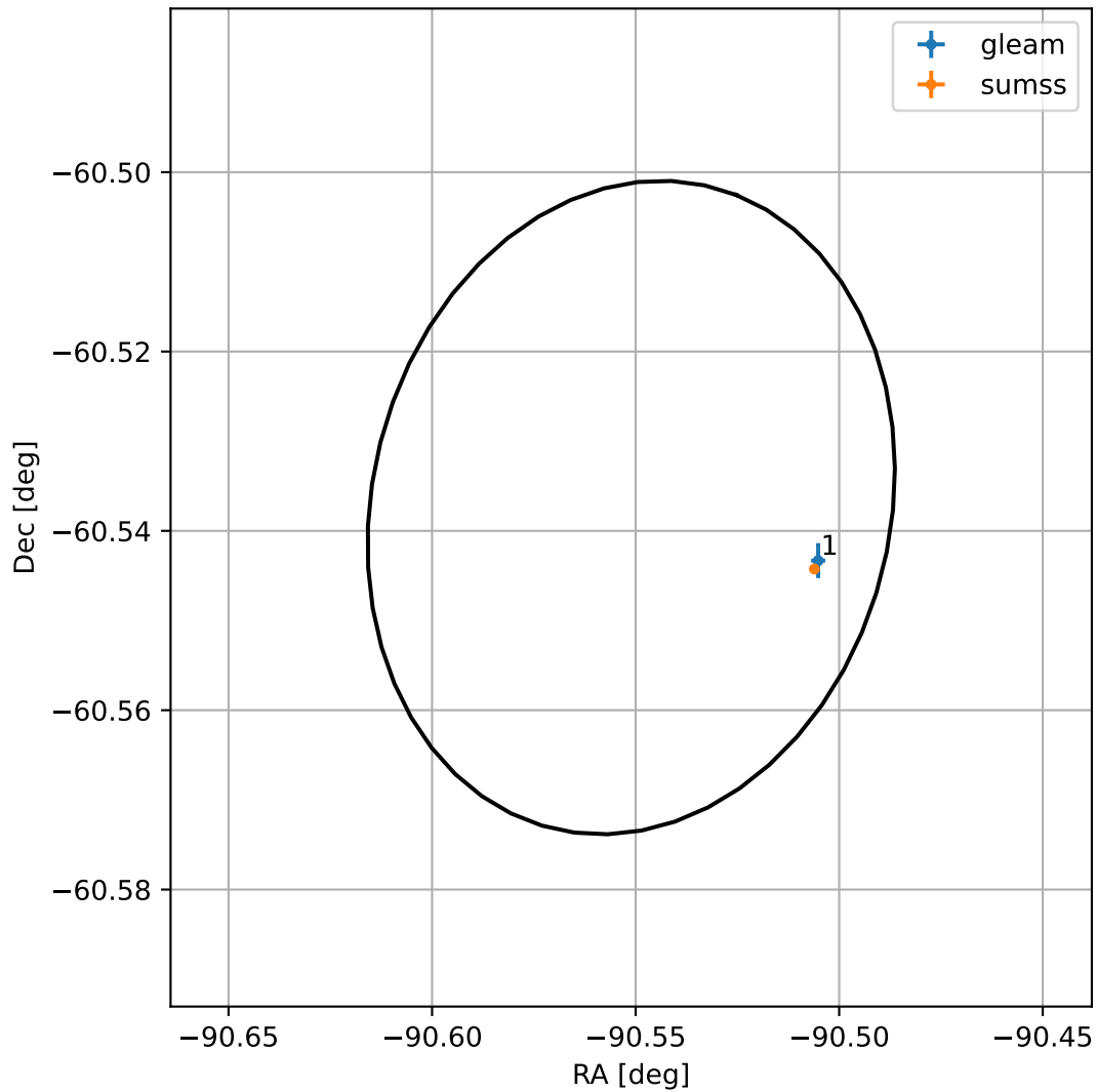
4FGL J1757.7-6032
