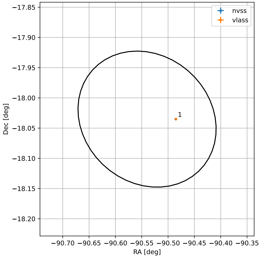
4FGL J1757.8-1802
