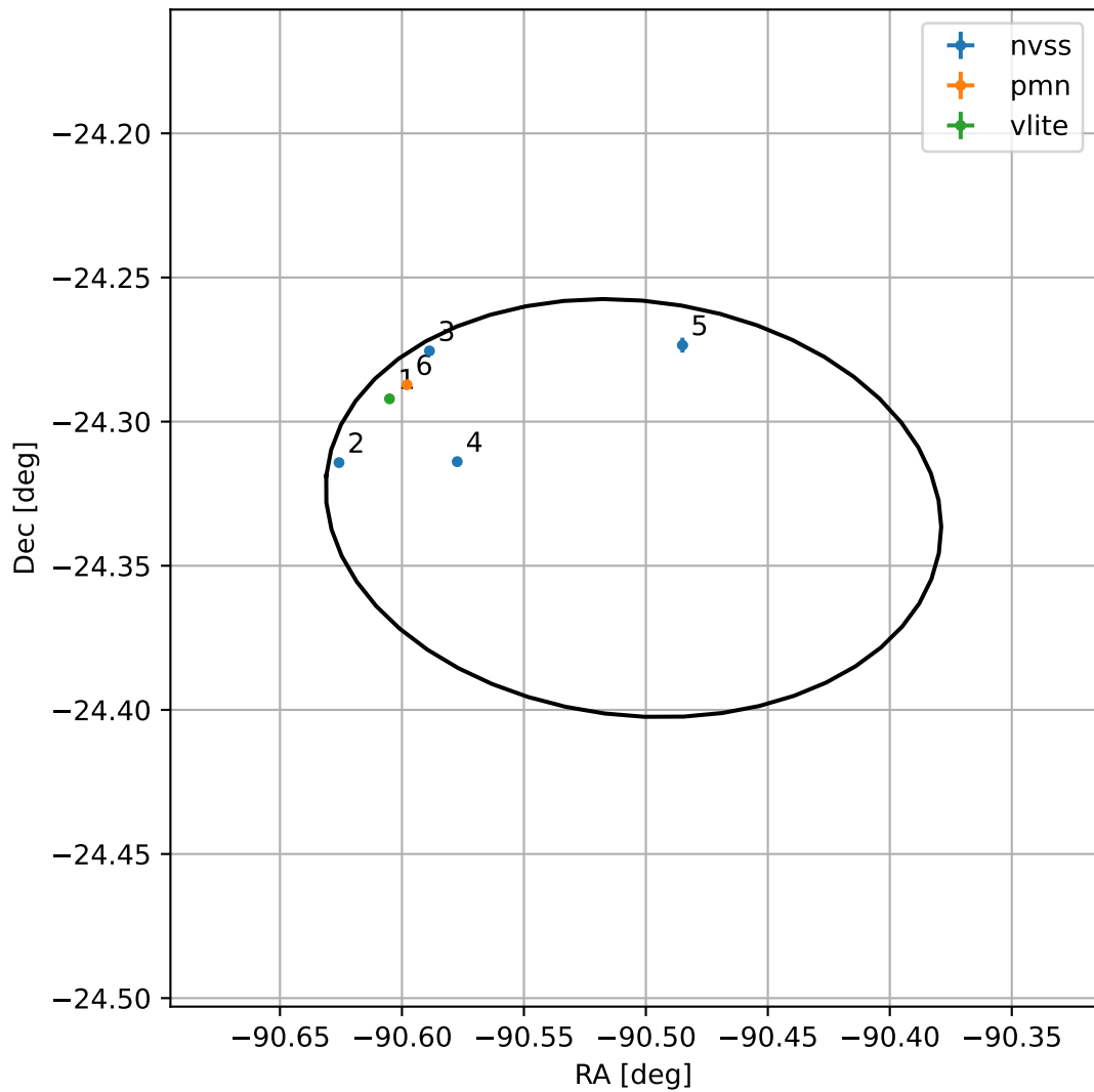
4FGL J1757.9-2419
