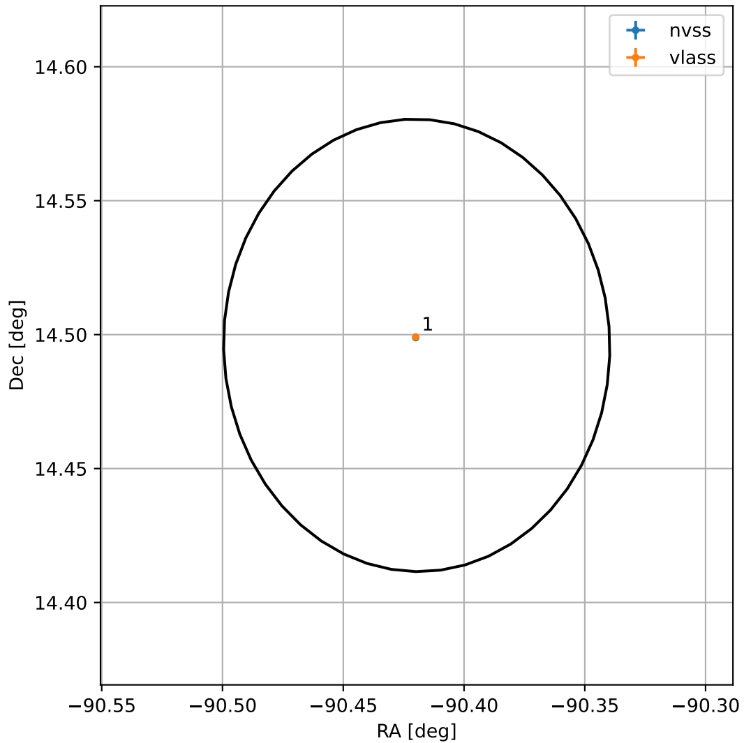
4FGL J1758.3+1429
