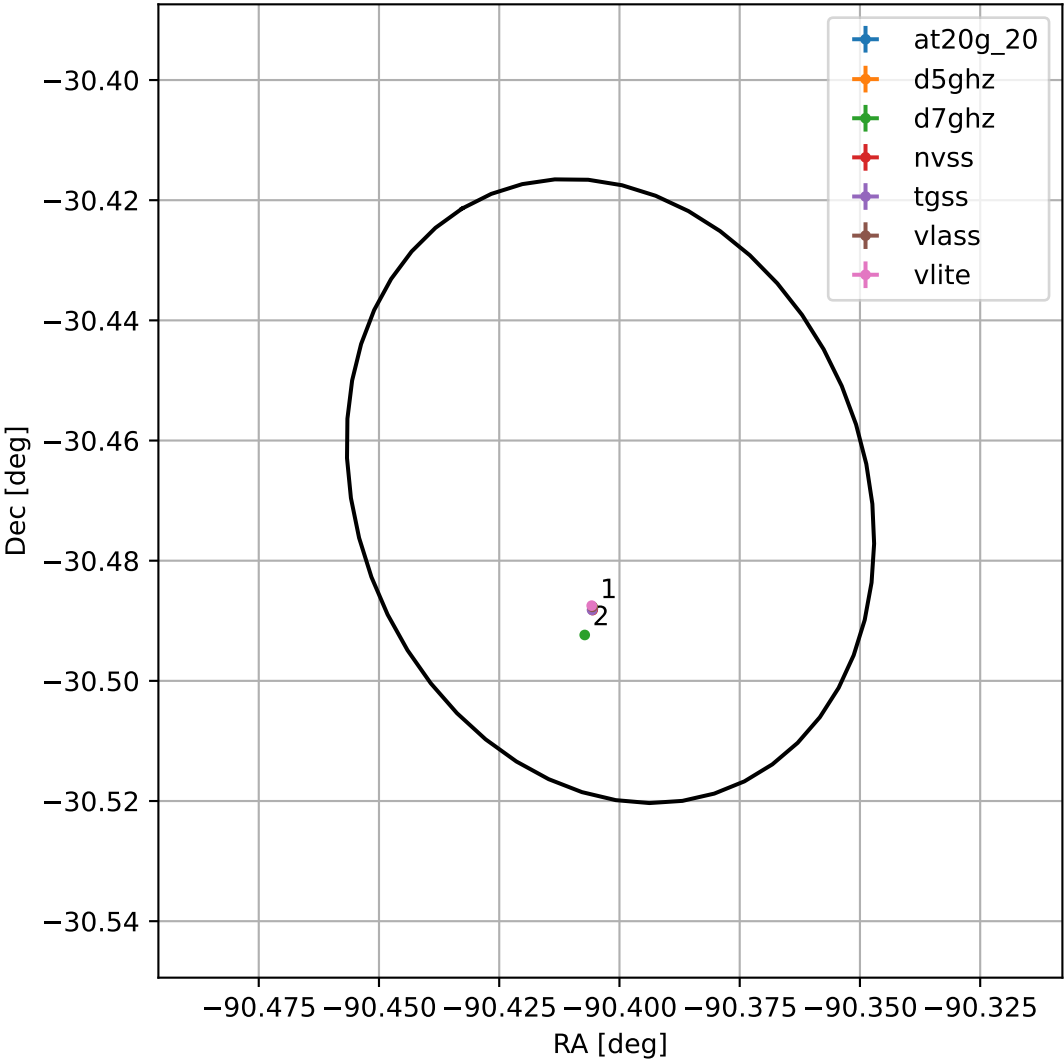
4FGL J1758.3-3028
