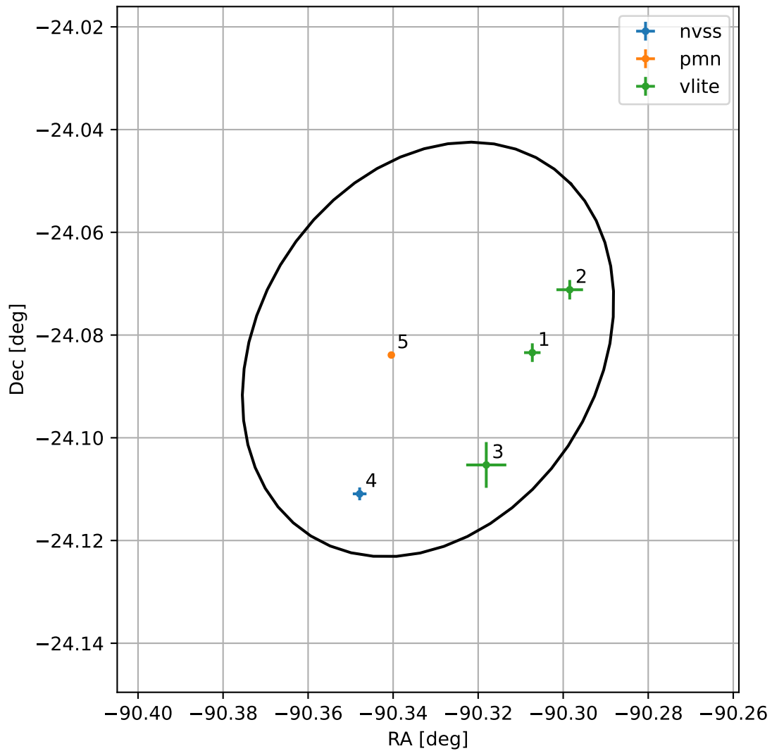
4FGL J1758.6-2404
