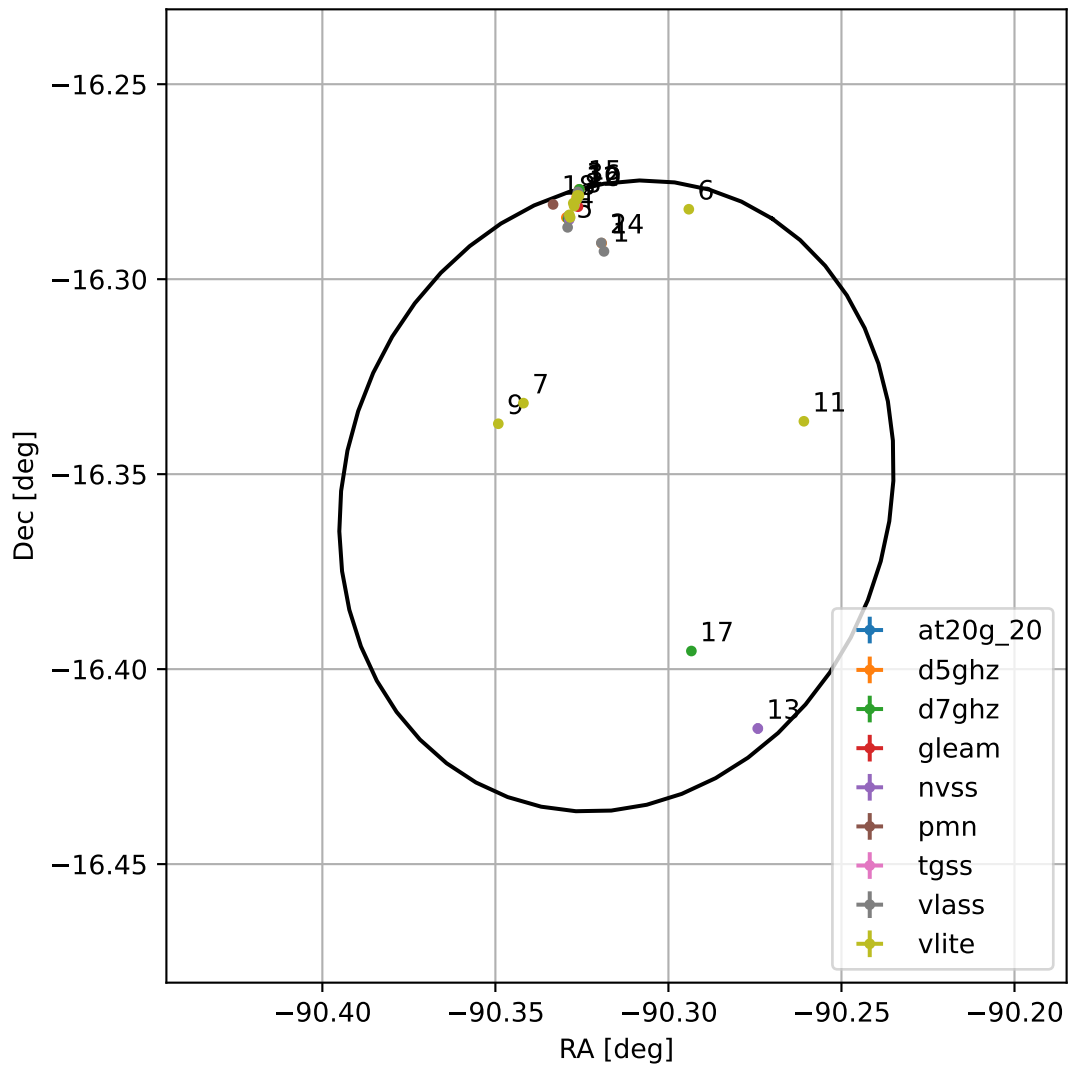
4FGL J1758.7-1621
