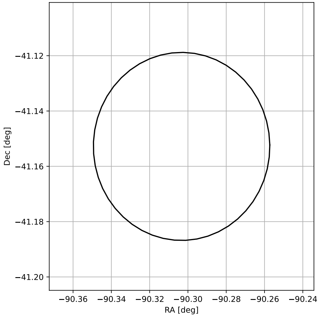
4FGL J1758.7-4109
