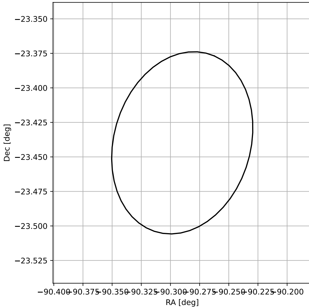
4FGL J1758.8-2326
