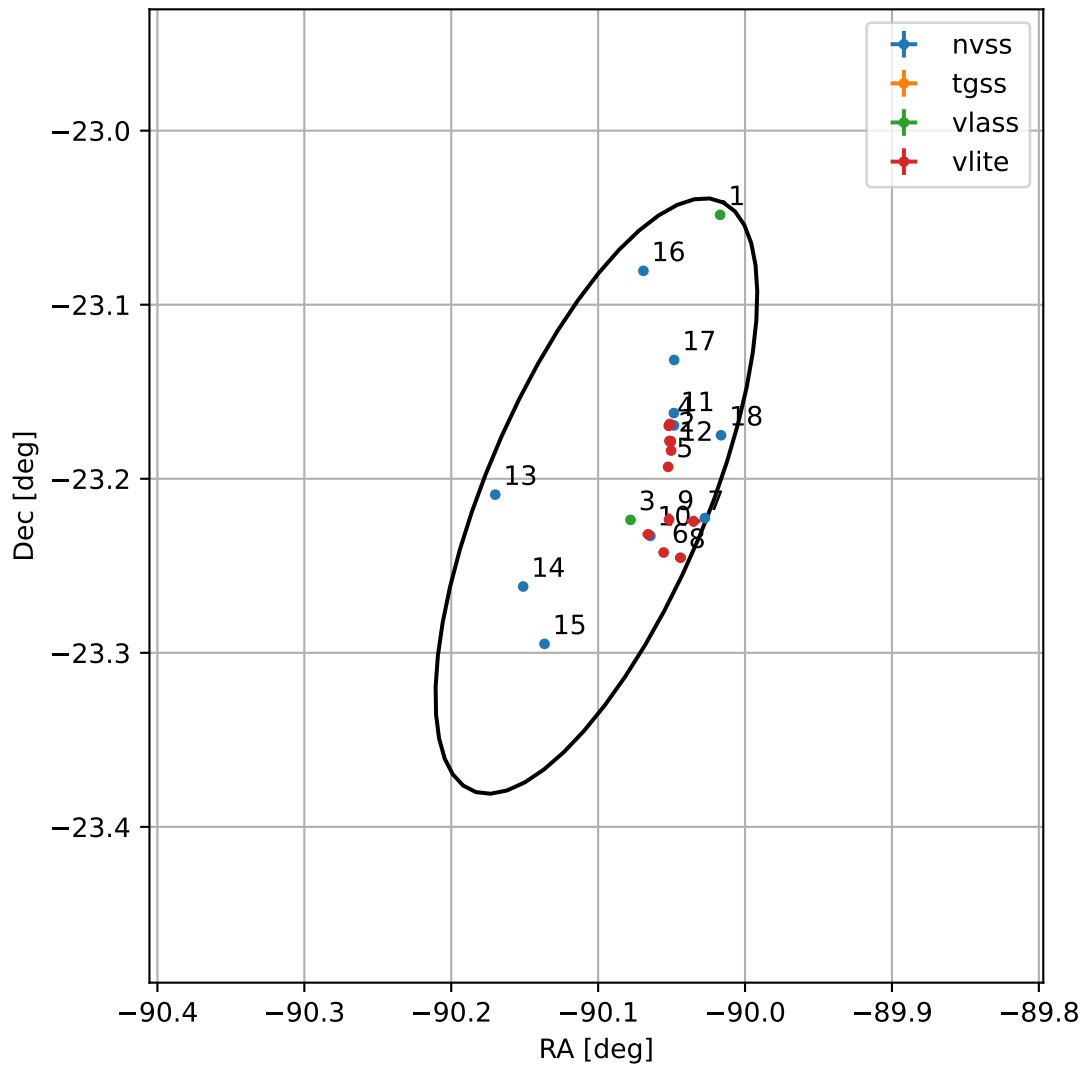
4FGL J1759.5-2312
