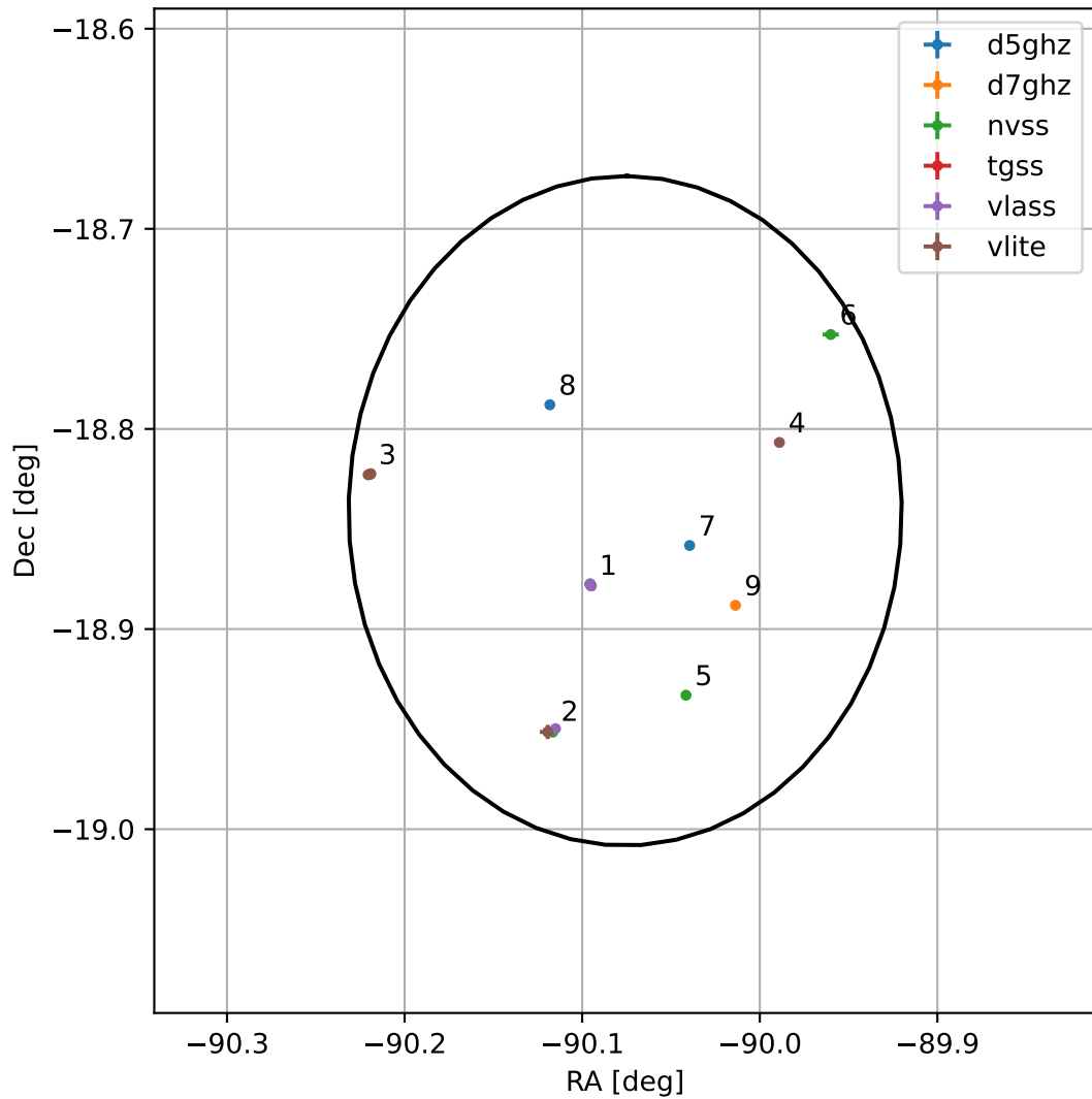
4FGL J1759.6-1850
