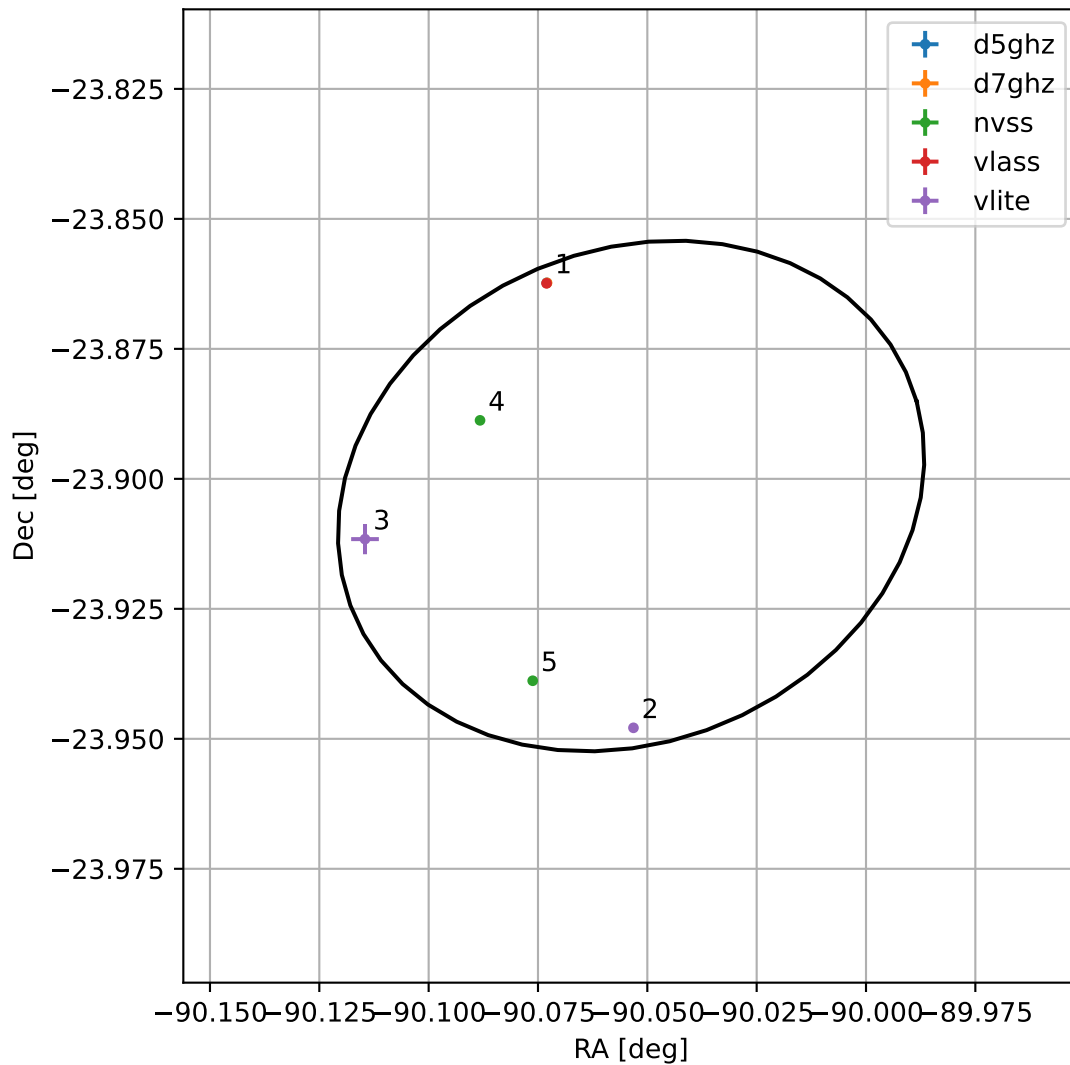
4FGL J1759.7-2354
