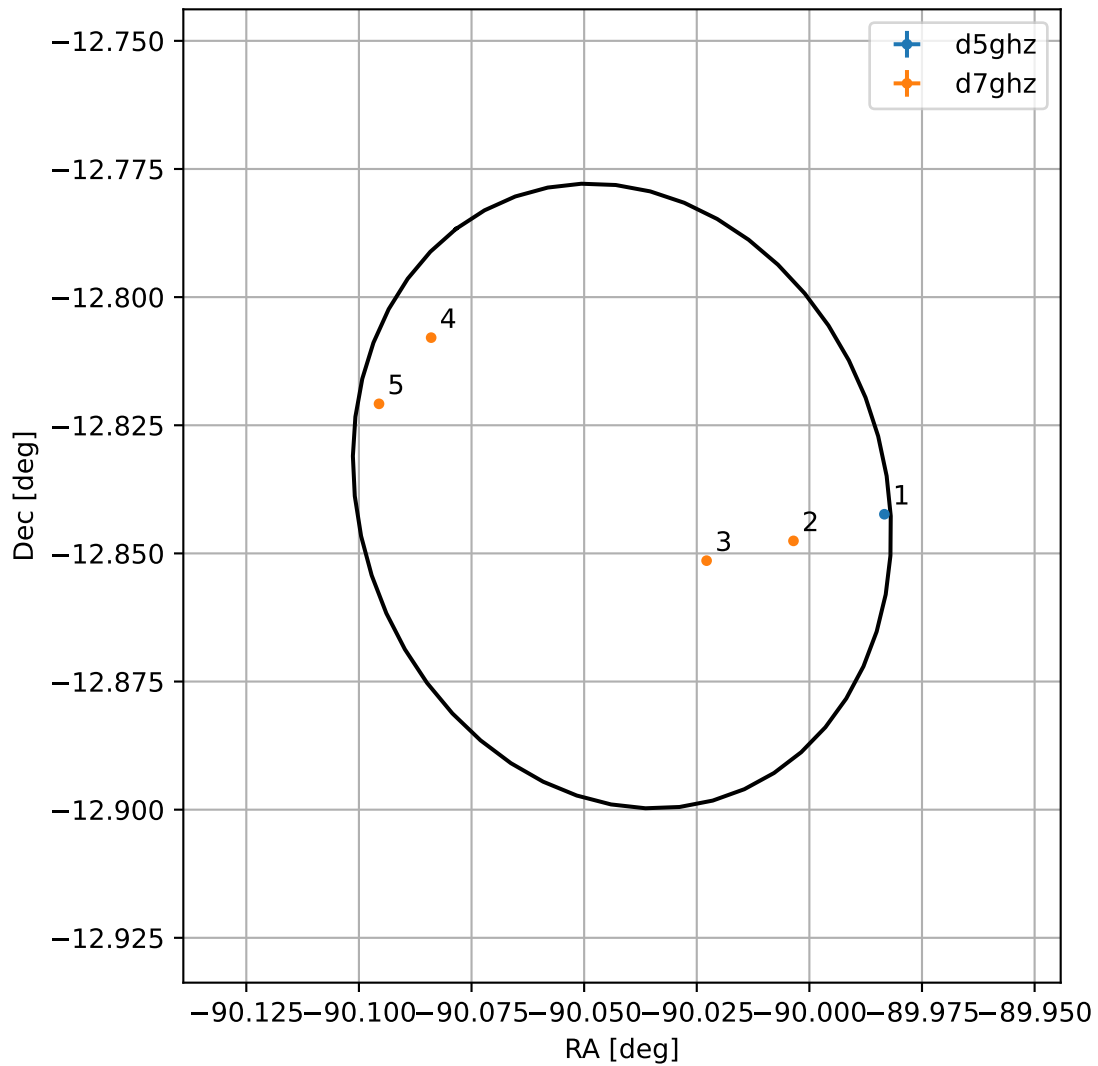
4FGL J1759.8-1250
