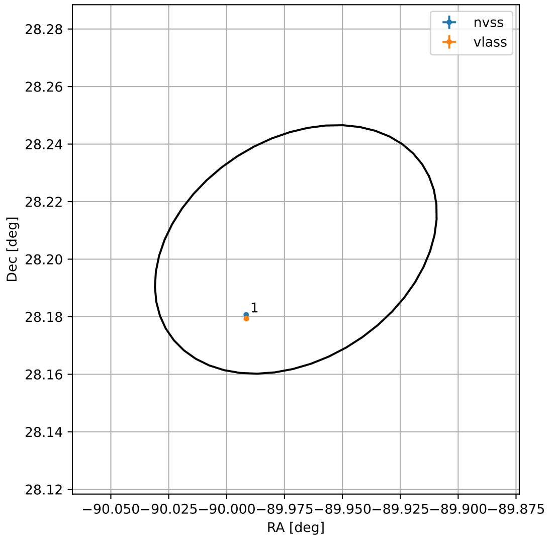
4FGL J1800.1+2812
