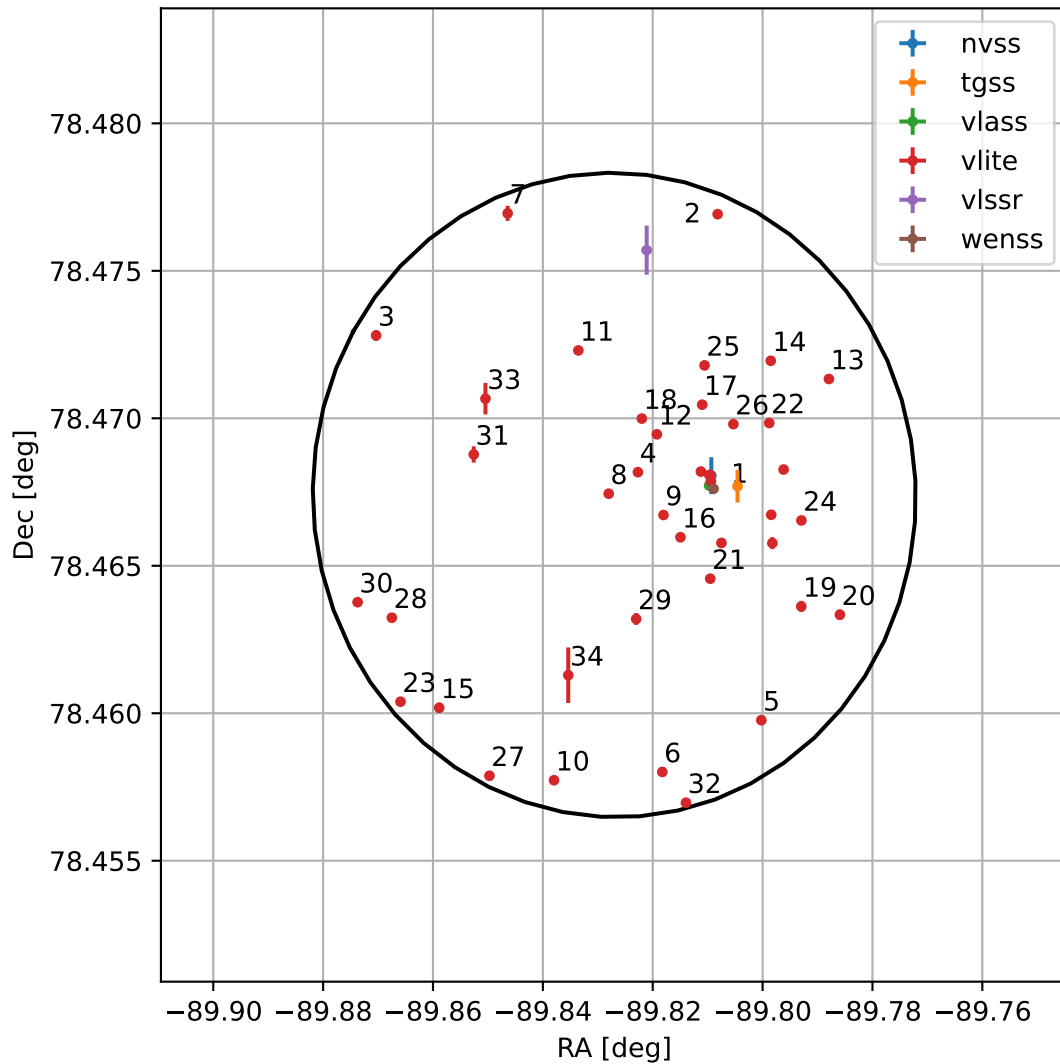
4FGL J1800.6+7828
