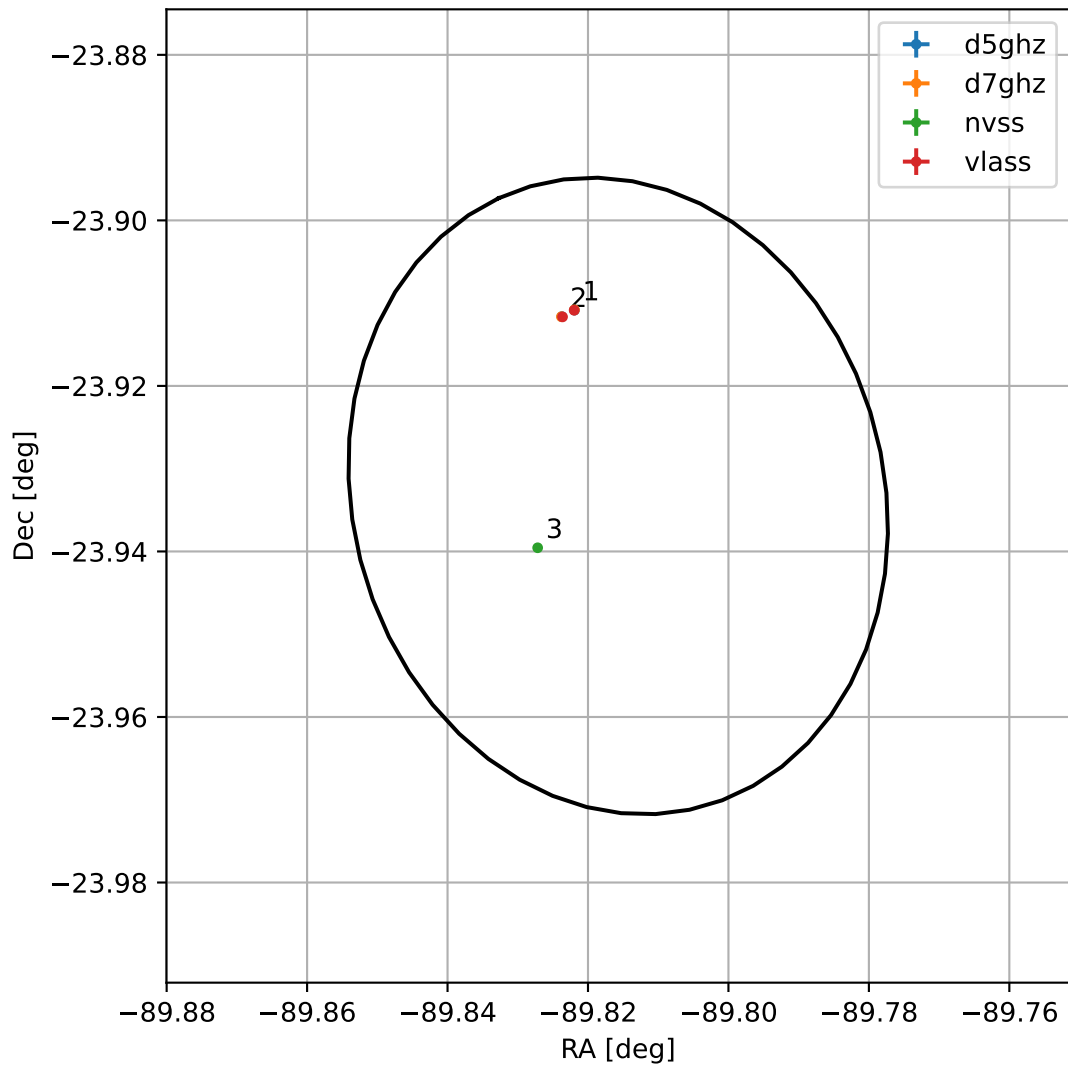
4FGL J1800.7-2355
