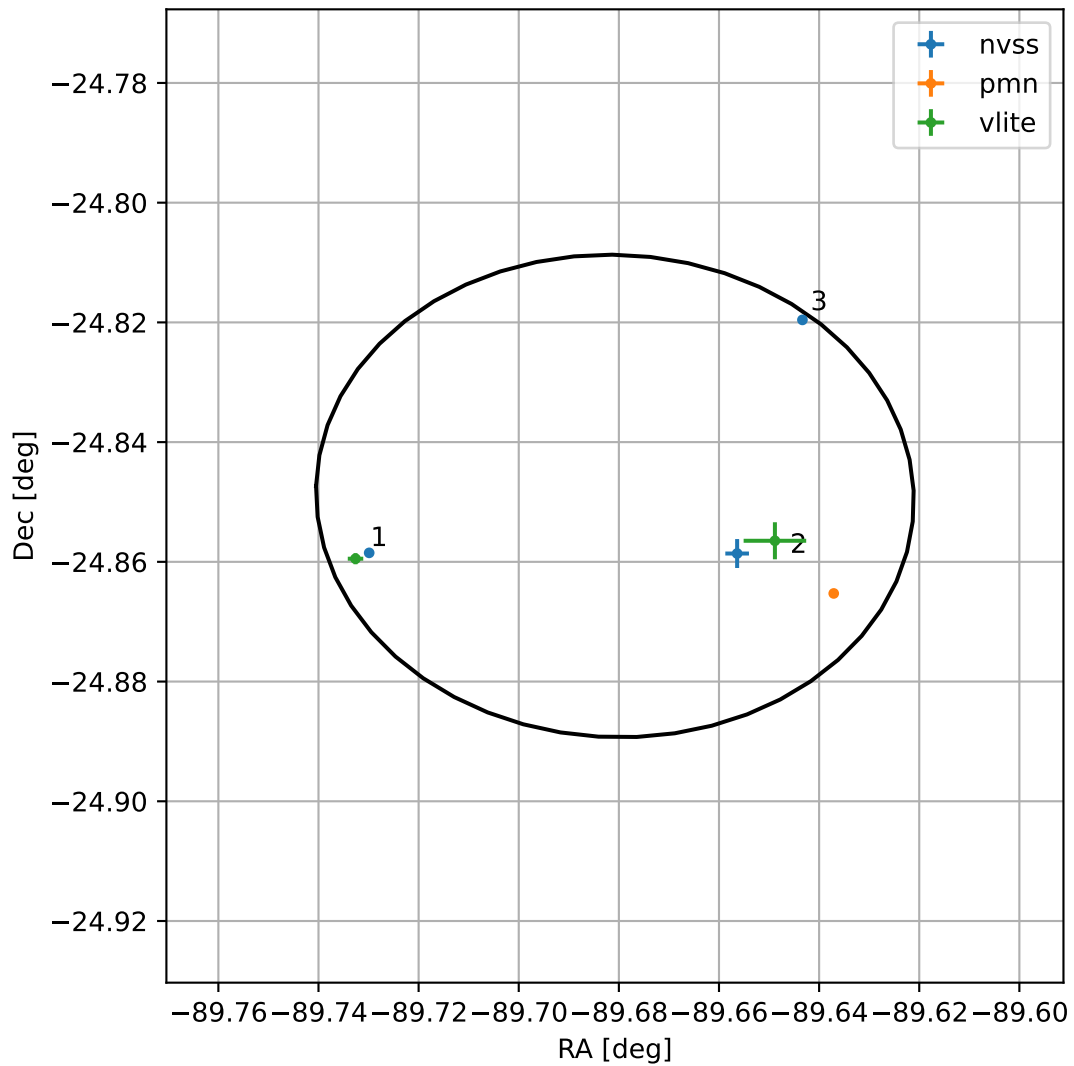
4FGL J1801.2-2450
