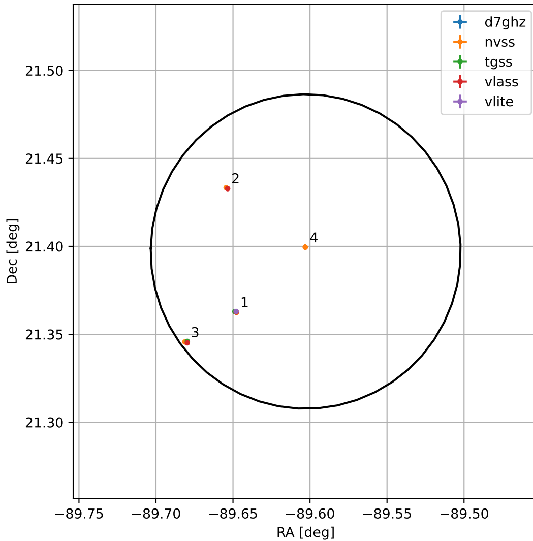
4FGL J1801.5+2123
