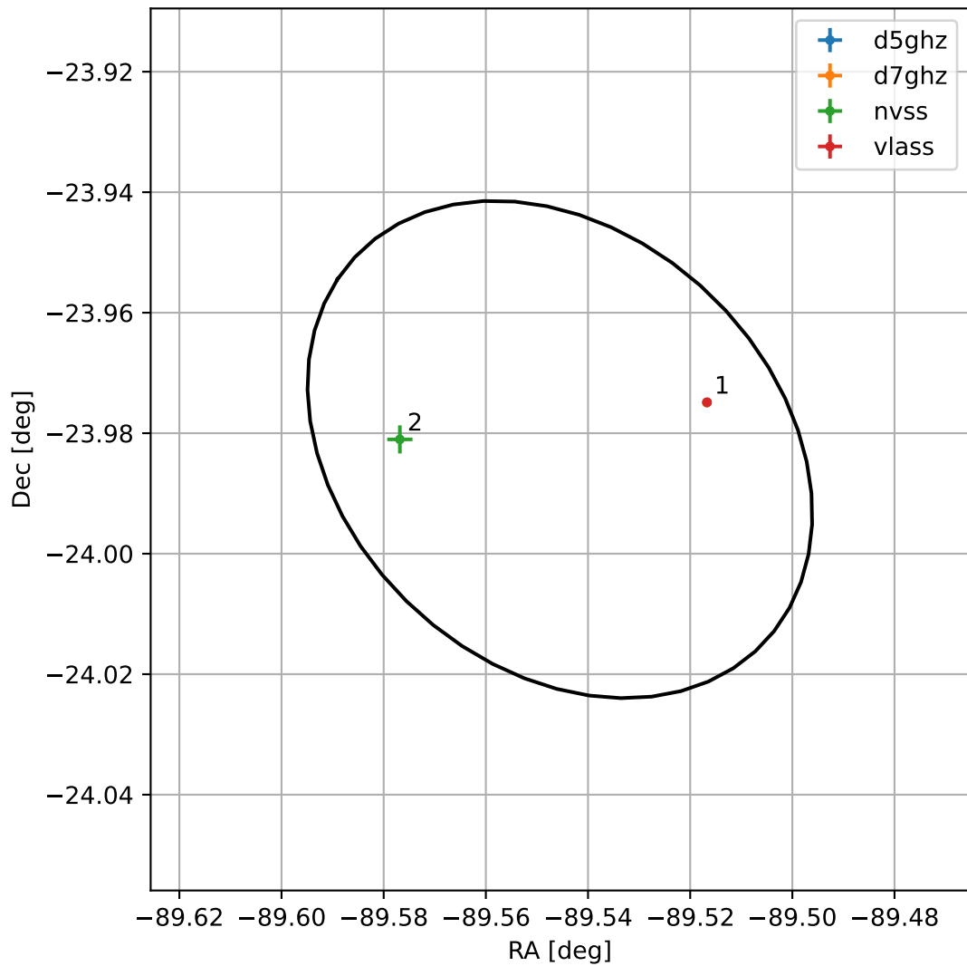
4FGL J1801.8-2358
