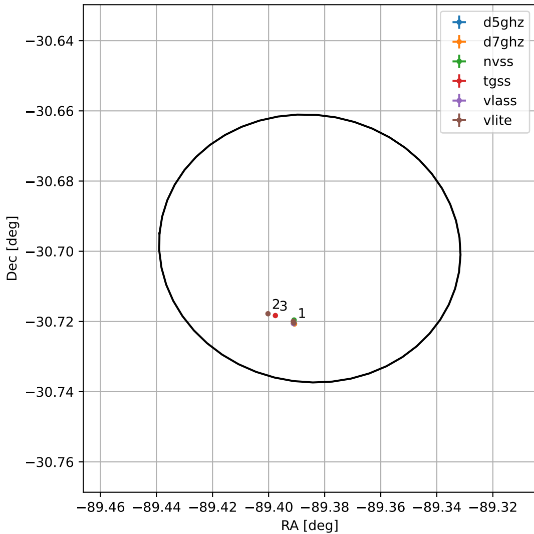
4FGL J1802.4-3041
