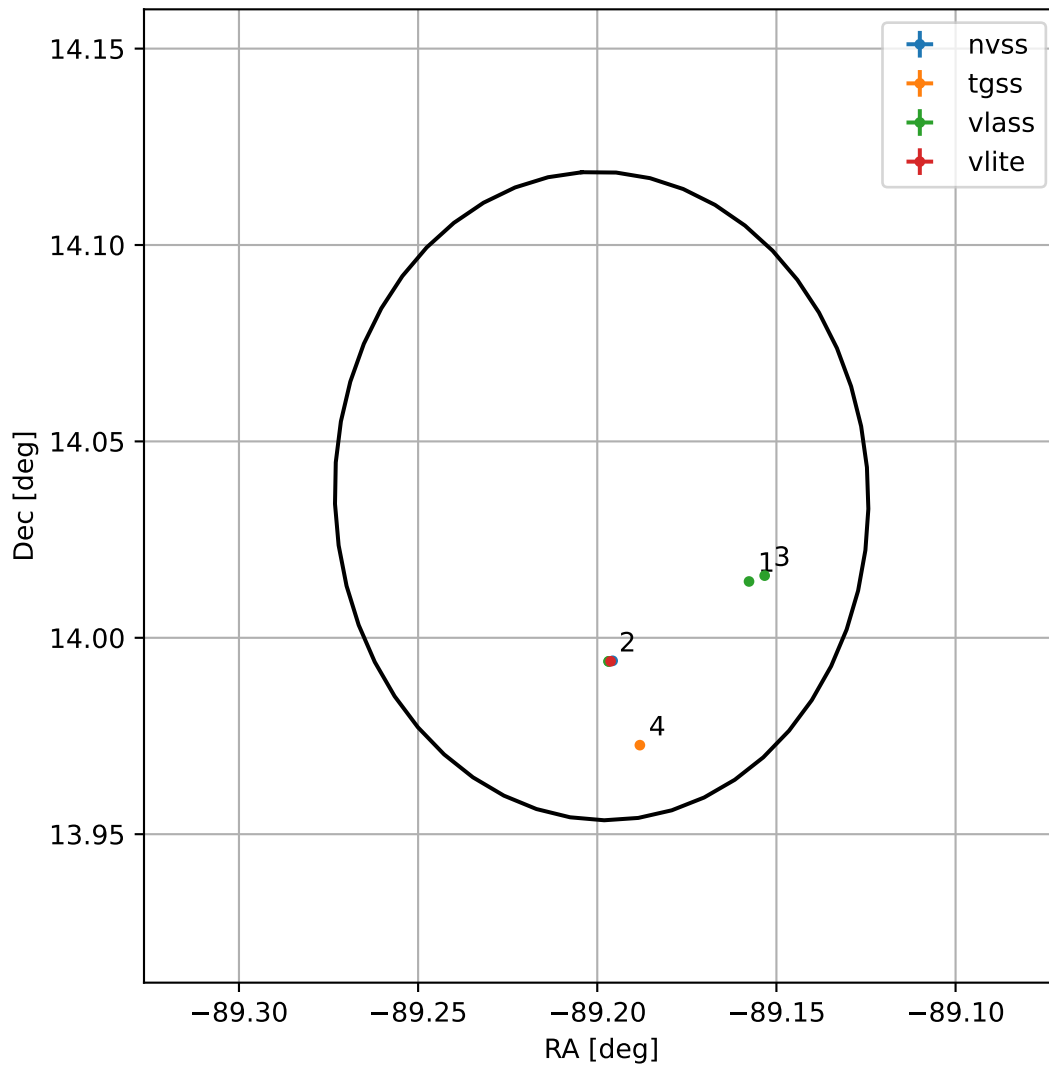
4FGL J1803.2+1402
