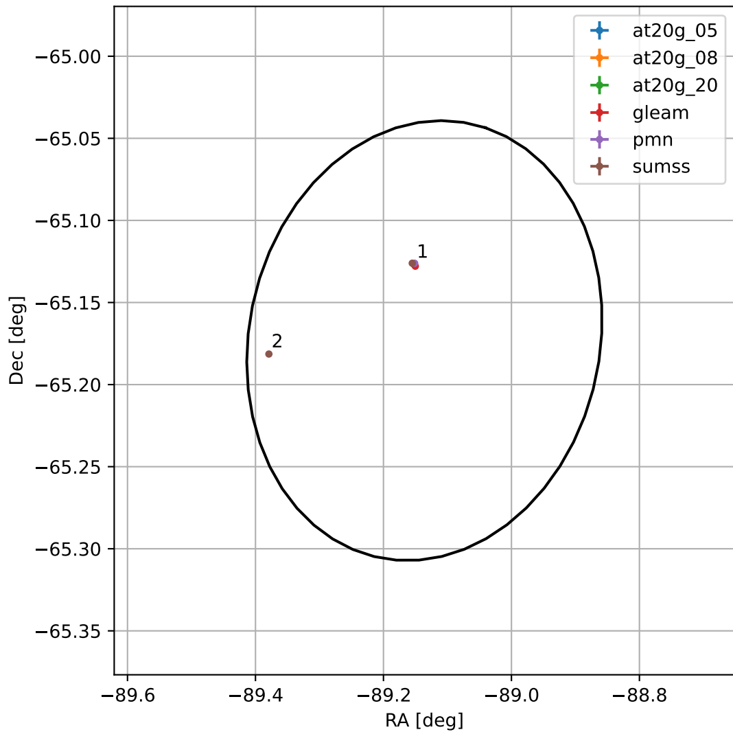
4FGL J1803.4-6510
