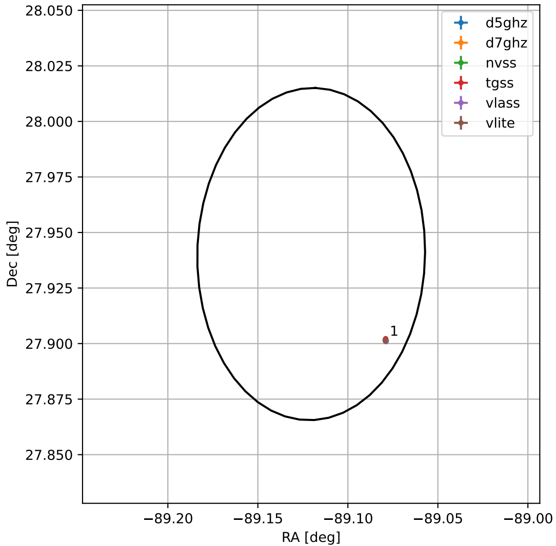
4FGL J1803.5+2756
