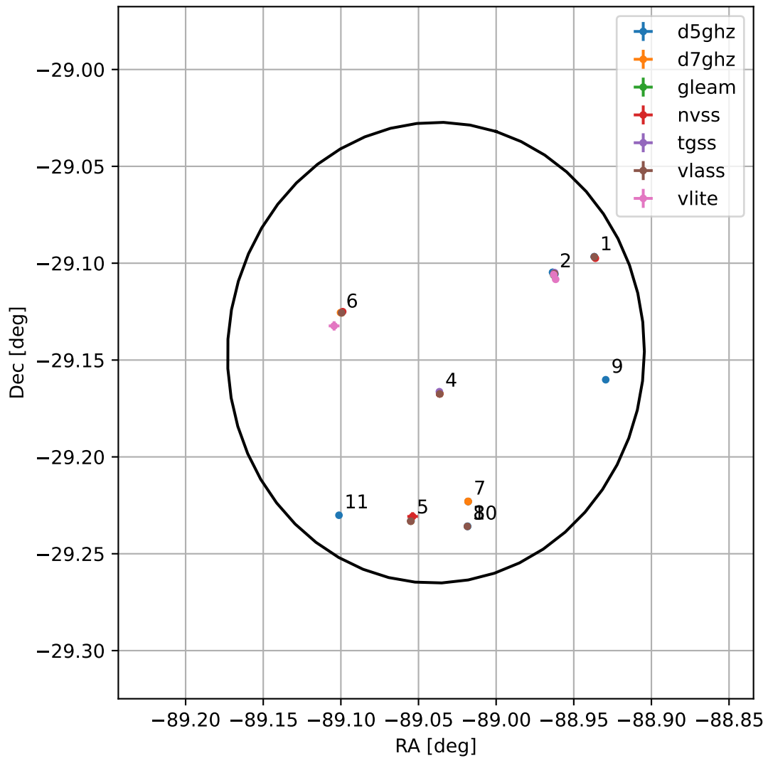
4FGL J1803.8-2908
