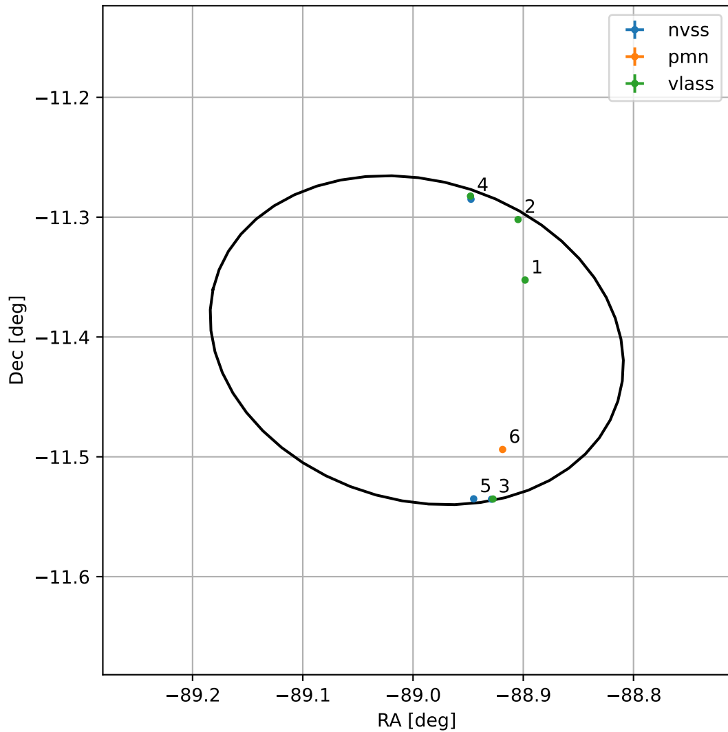
4FGL J1804.0-1124
