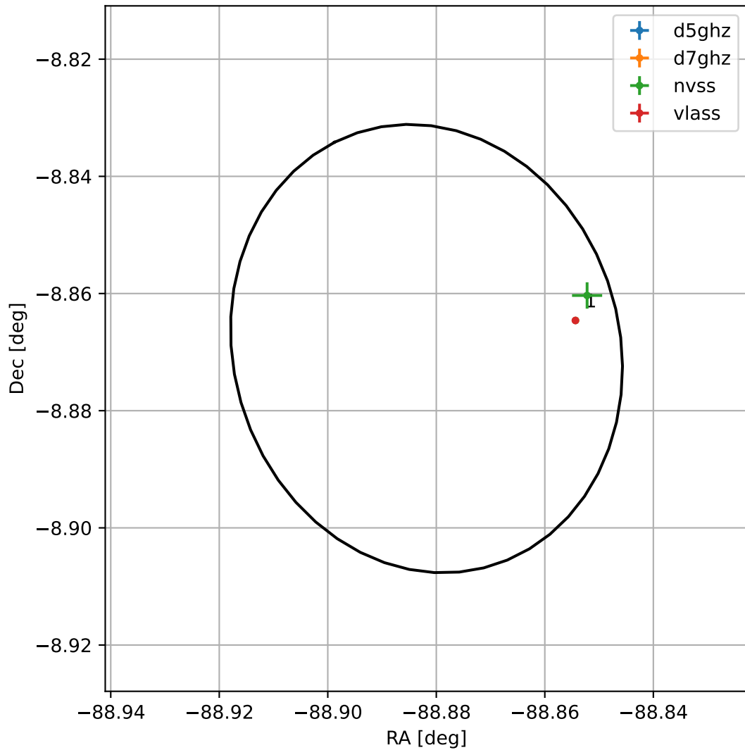
4FGL J1804.4-0852
