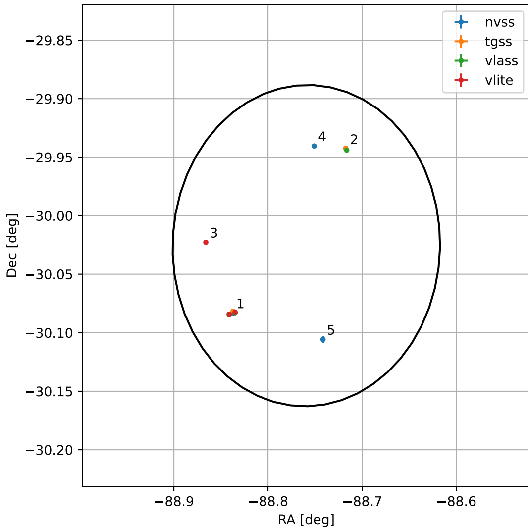
4FGL J1804.9-3001
