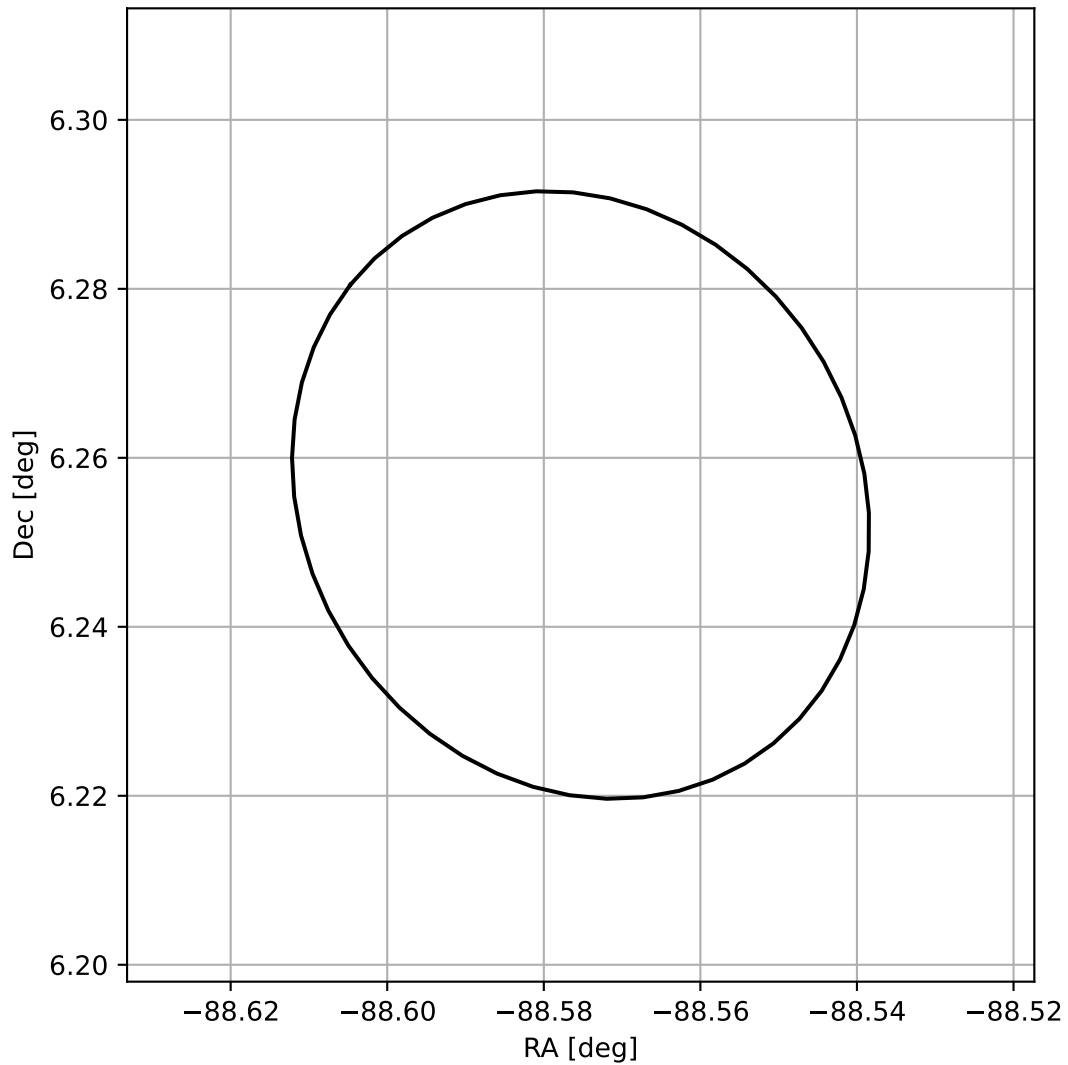
4FGL J1805.6+0615
