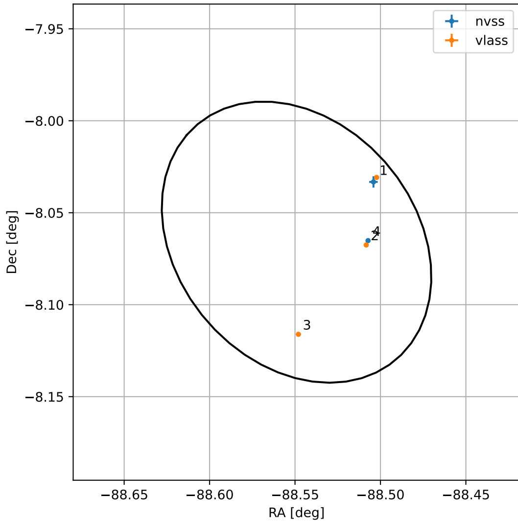
4FGL J1805.8-0803
