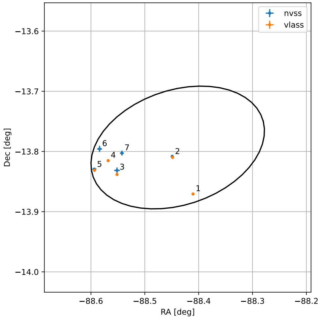
4FGL J1806.2-1347
