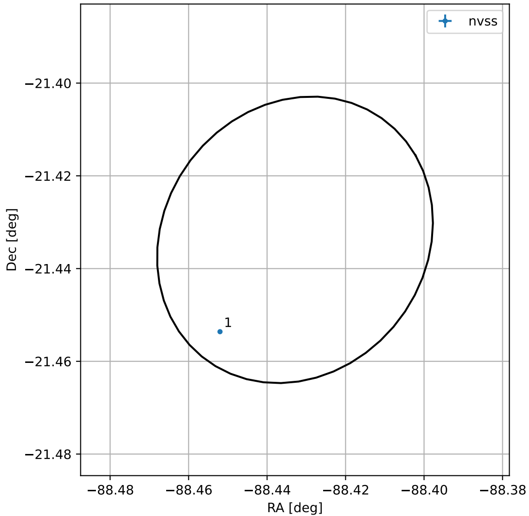
4FGL J1806.2-2126
