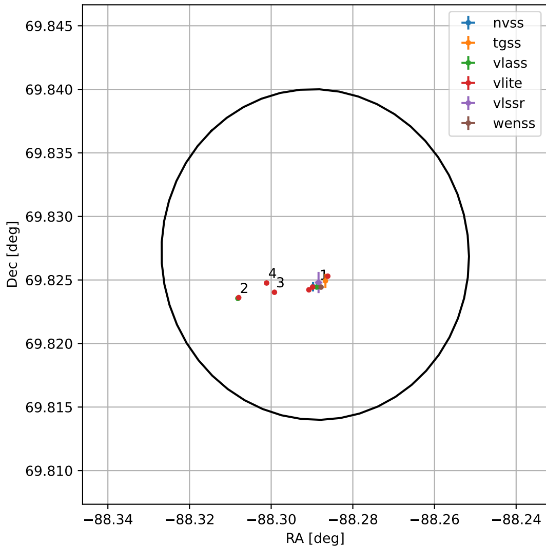
4FGL J1806.8+6949
