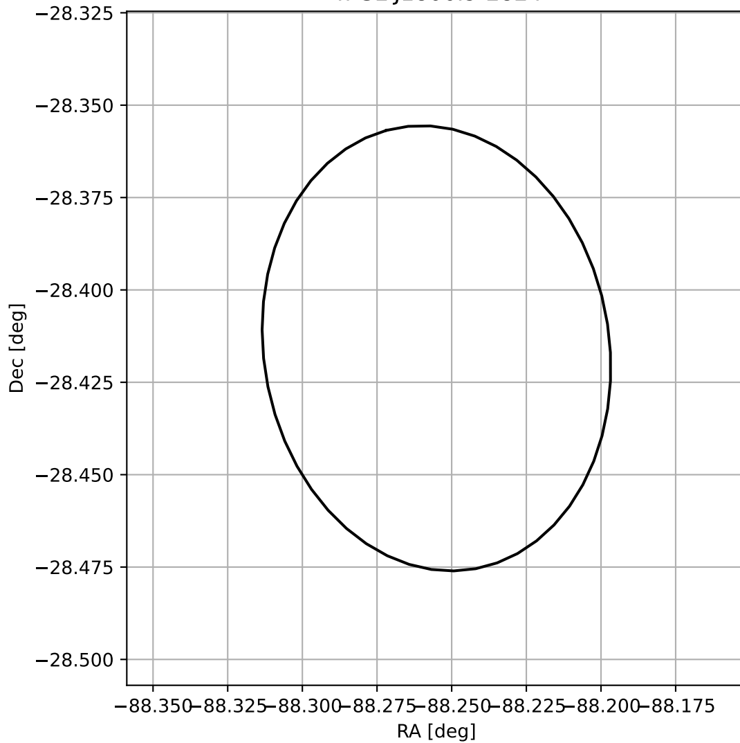
4FGL J1806.9-2824
