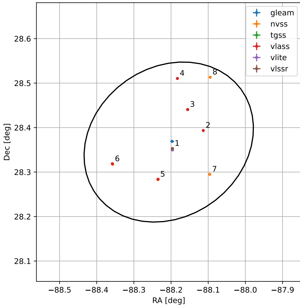
4FGL J1807.1+2822
