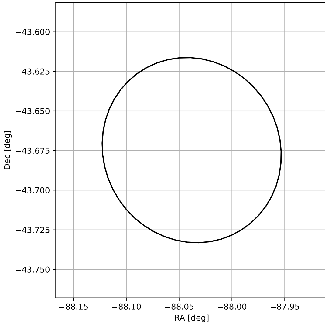
4FGL J1807.8-4340
