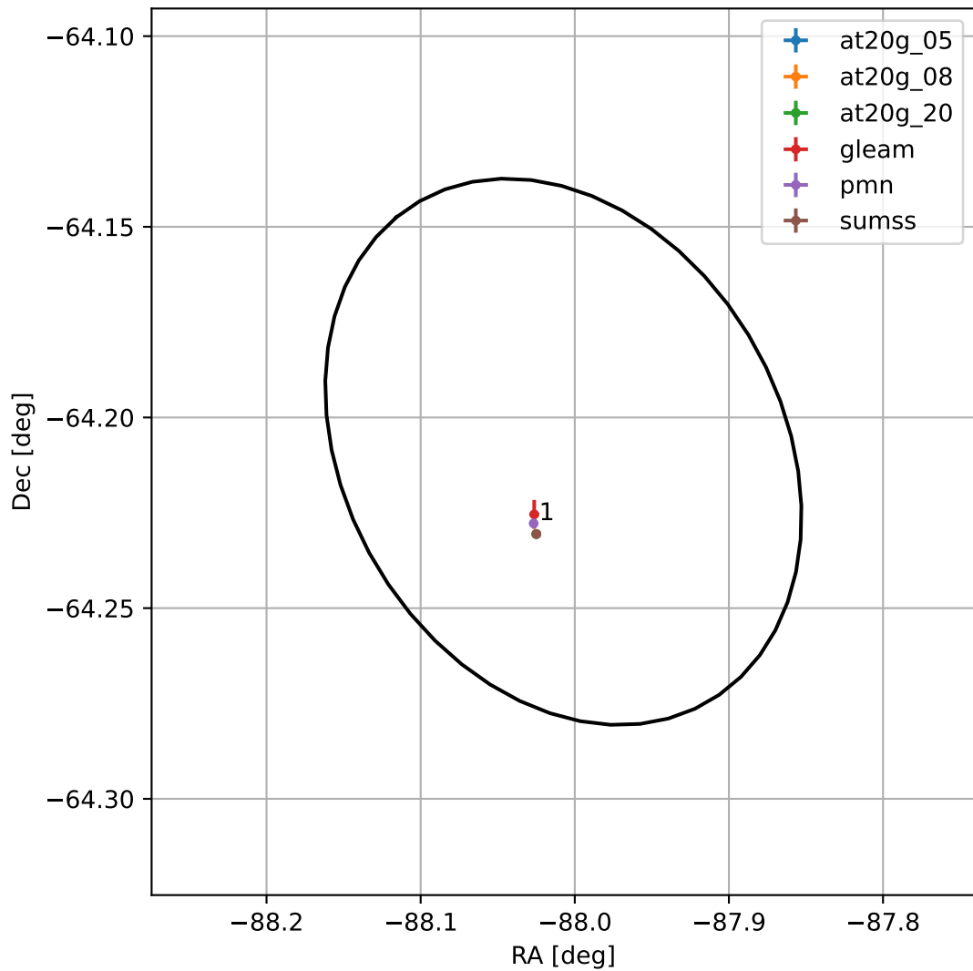
4FGL J1807.9-6412
