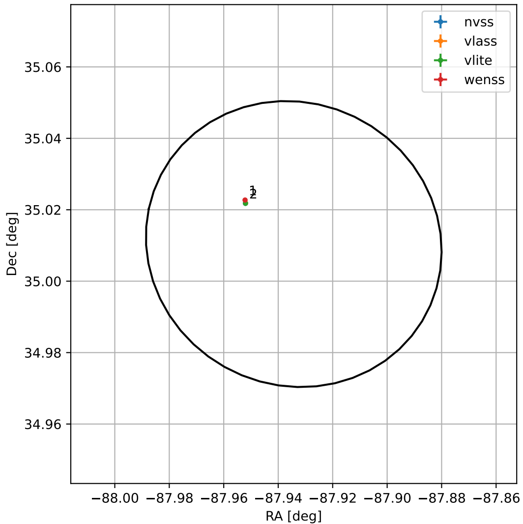
4FGL J1808.2+3500
