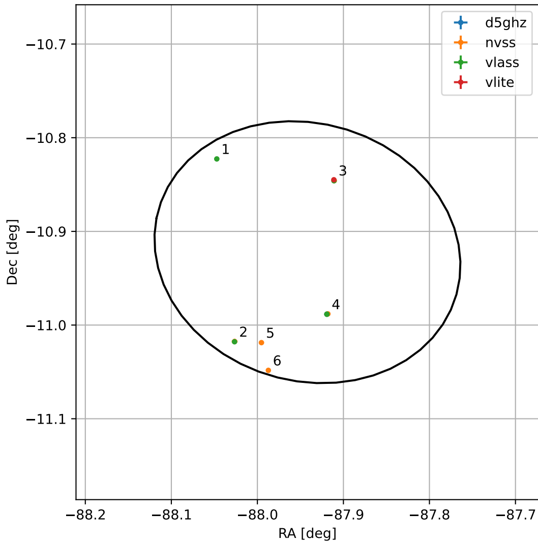
4FGL J1808.2-1055
