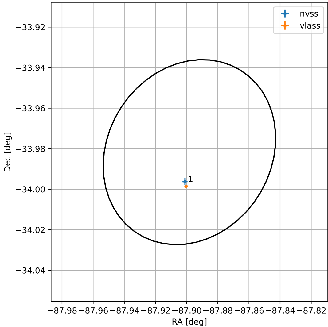
4FGL J1808.4-3358
