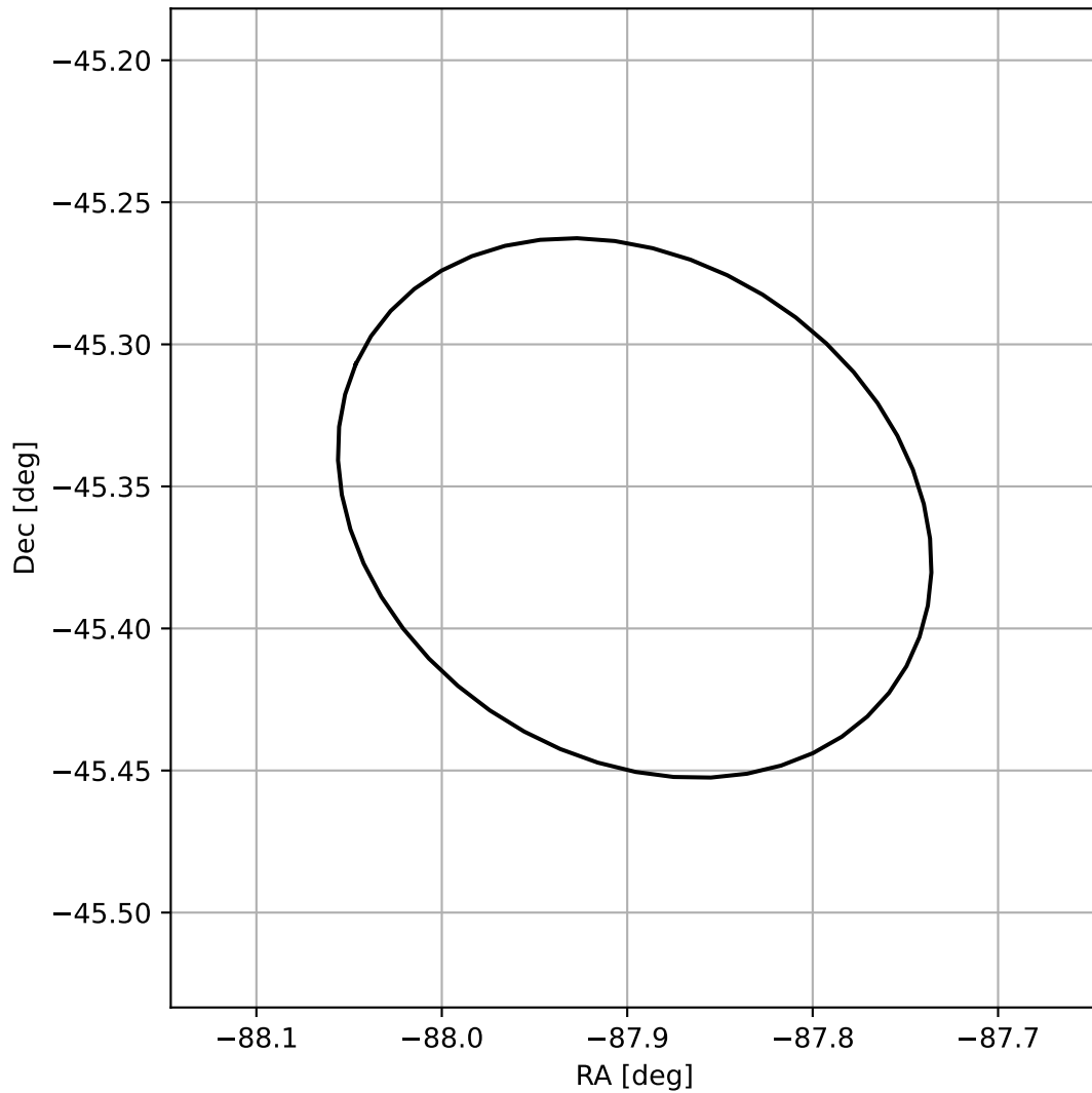
4FGL J1808.4-4521
