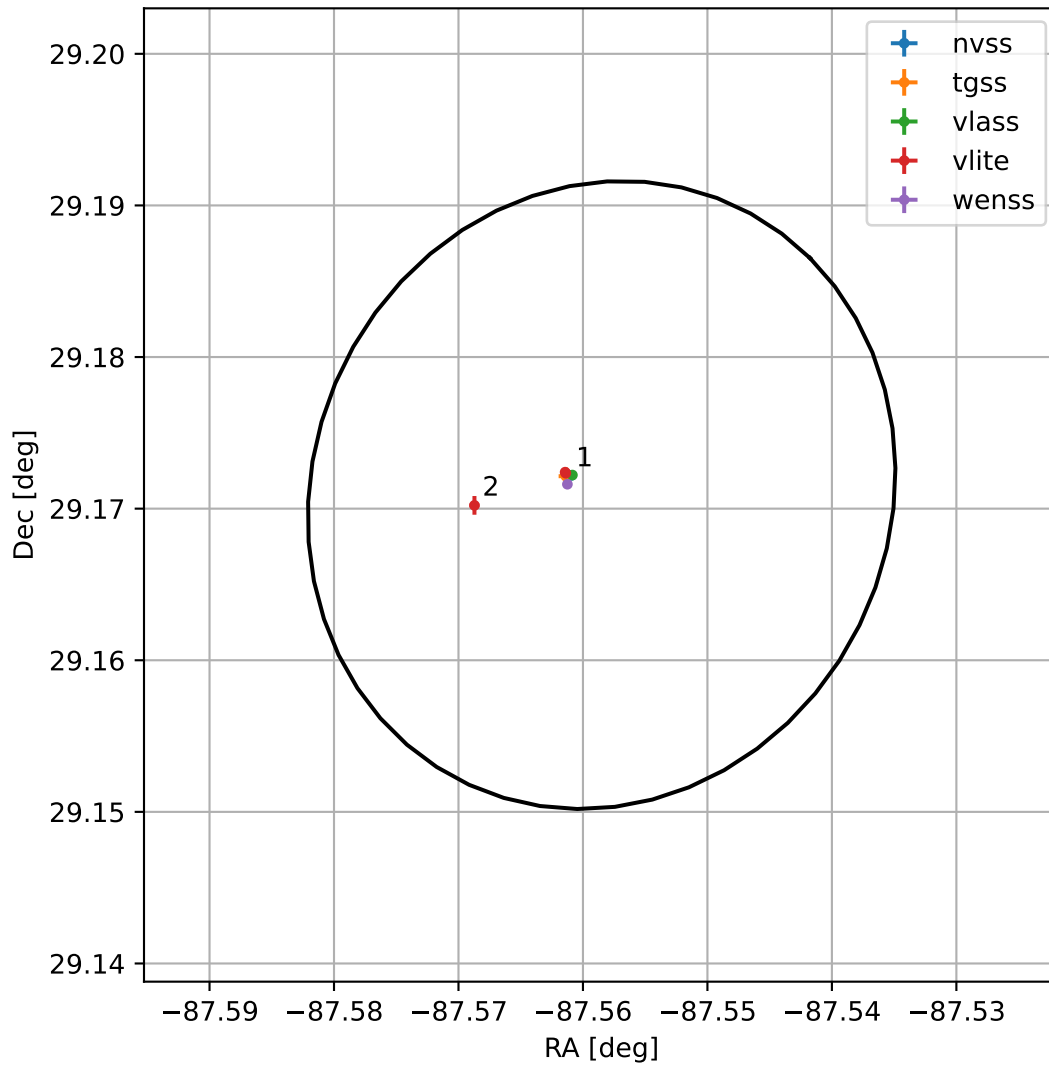
4FGL J1809.7+2910
