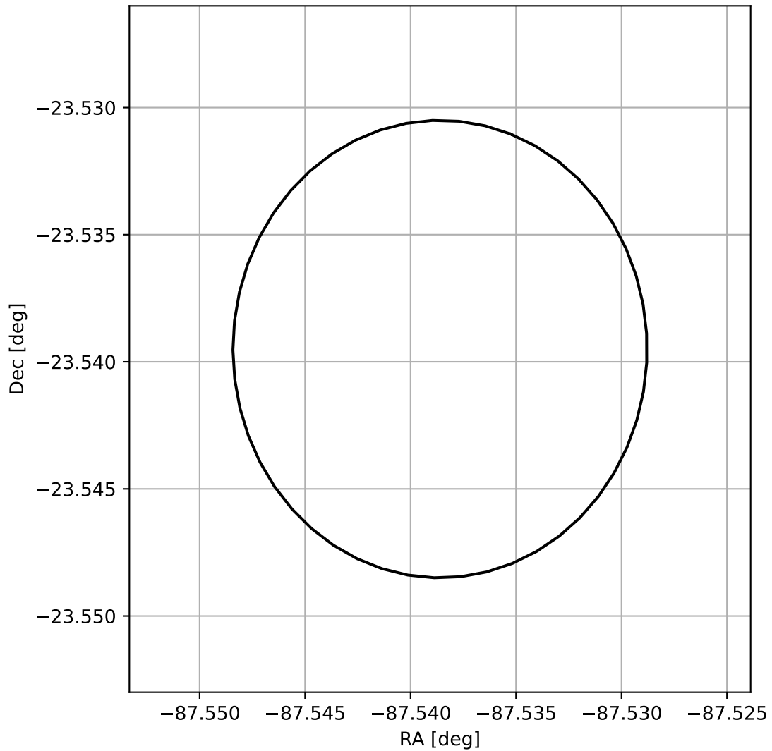
4FGL J1809.8-2332
