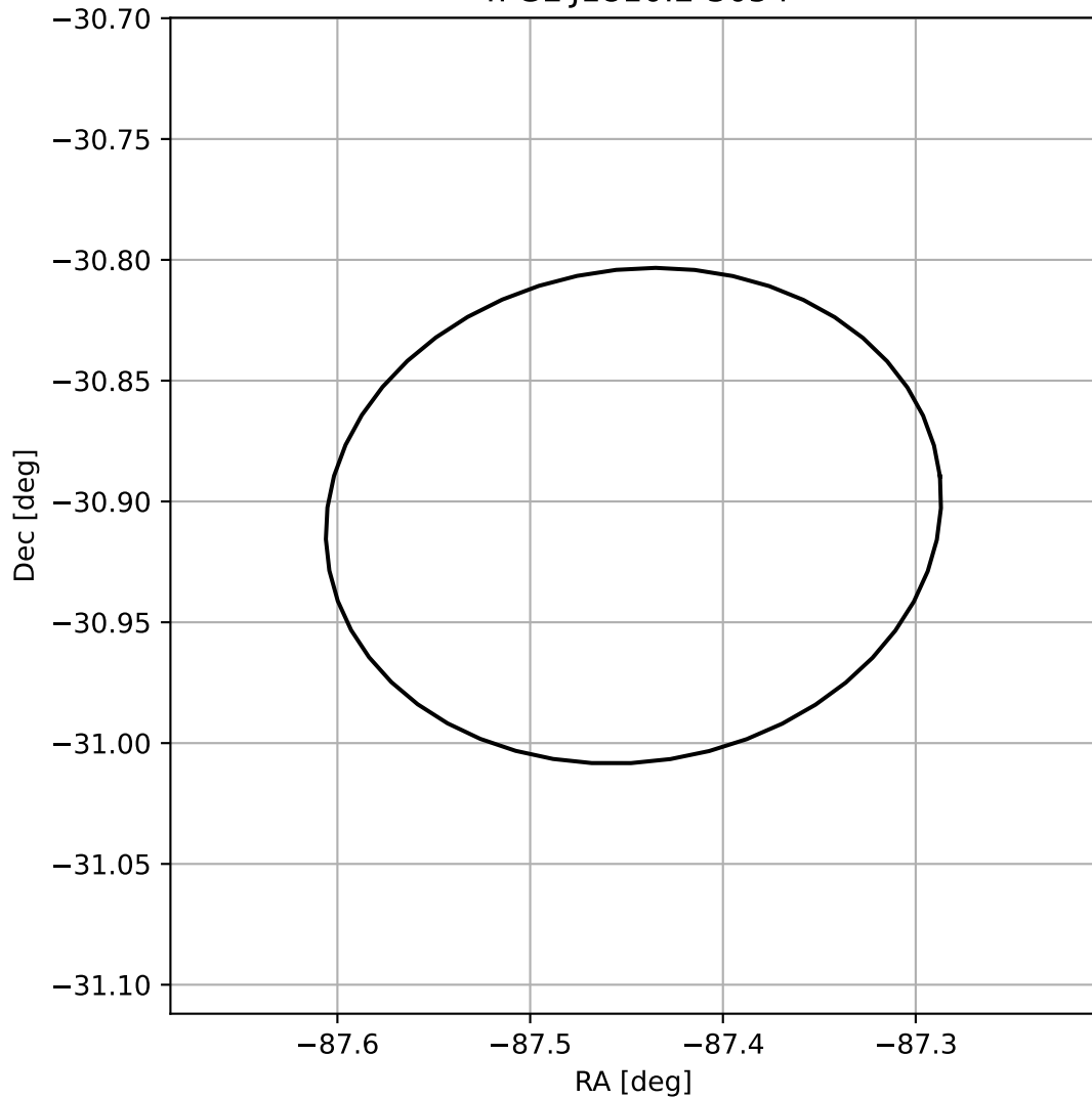
4FGL J1810.2-3054
